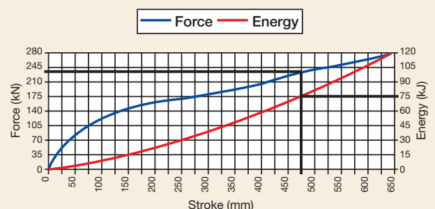
120 kJ Double Bar Technogrid
