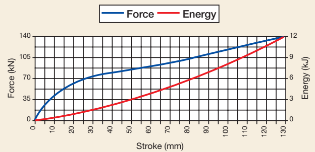
12 kJ Double Bar Technogrid
