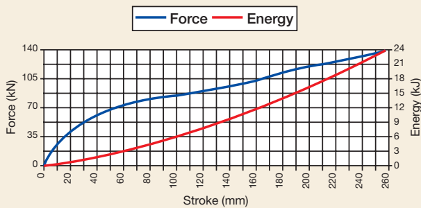
24 kJ Double Bar Technogrid
