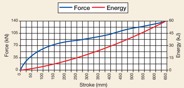
60 kJ Double Bar Technogrid
